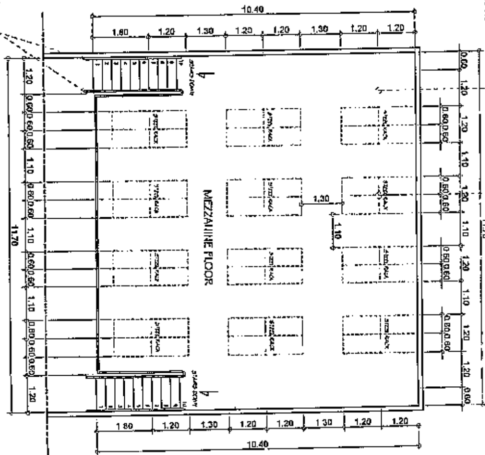
2 MEZZANINE FLOOR PLAN SCALE 1:100 MTRS.
