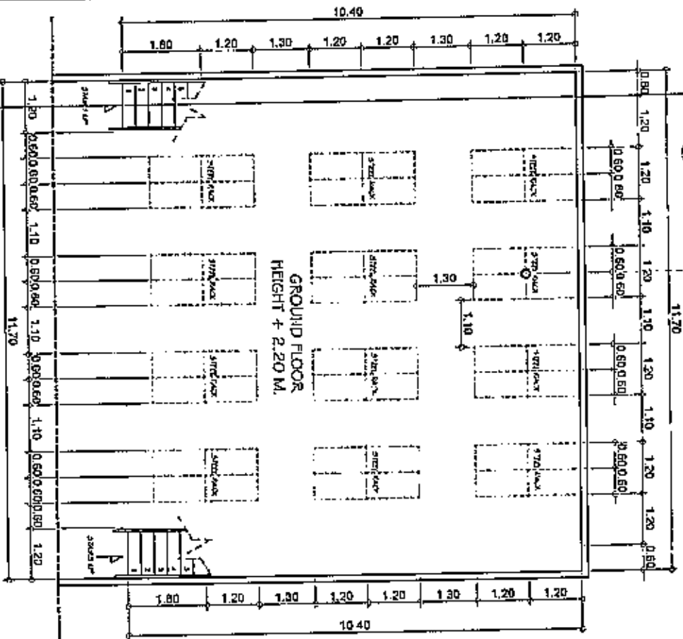
1 GROUND FLOOR PLAN SCALE 1:100 MTRS.
